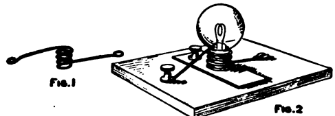
Wire Socket
