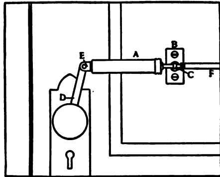
Pneumatic Door-Opener
