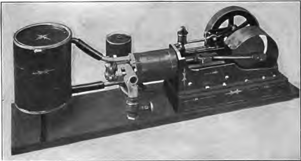
Complete Homemade Gasoline Engine
