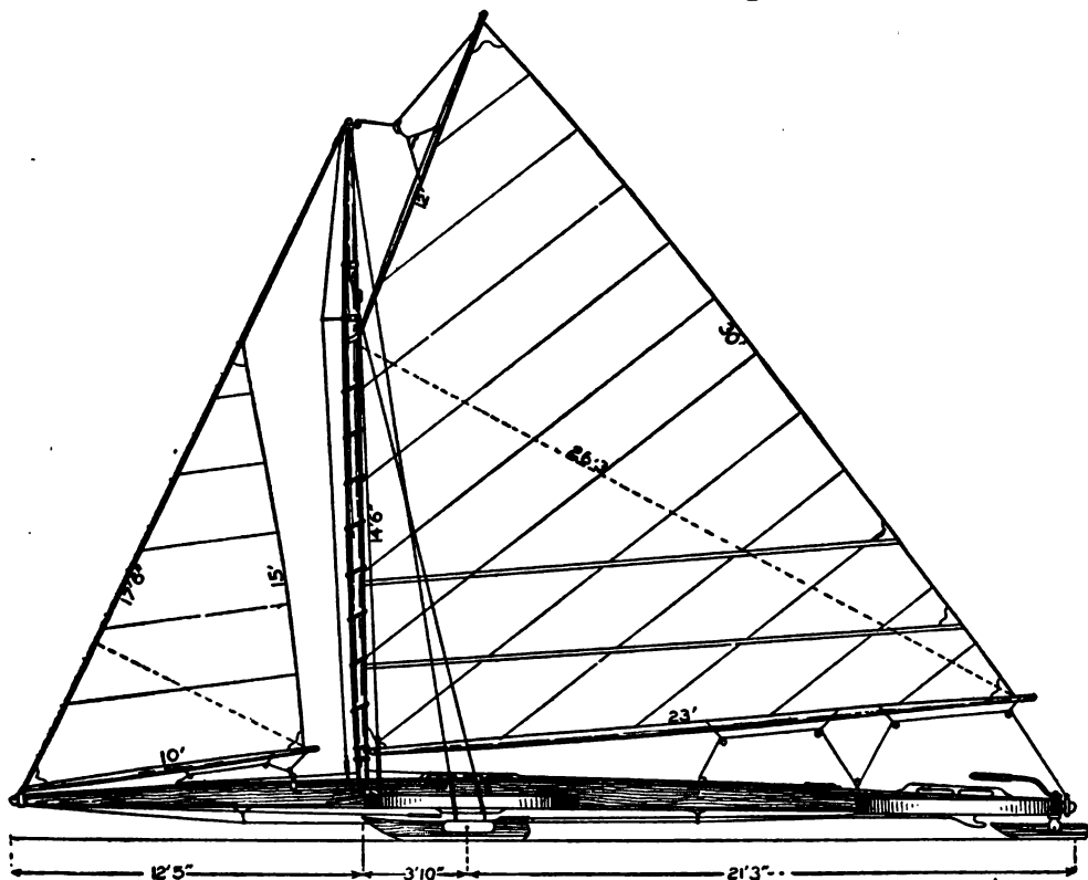
FIG. 1 Ice-Yacht Complete
