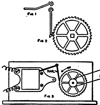
Novel Electric Motor
