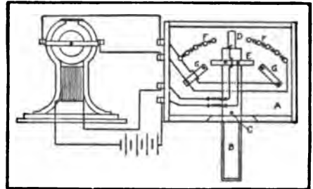
Reverse for Motor
