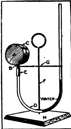
Air Thermometer
