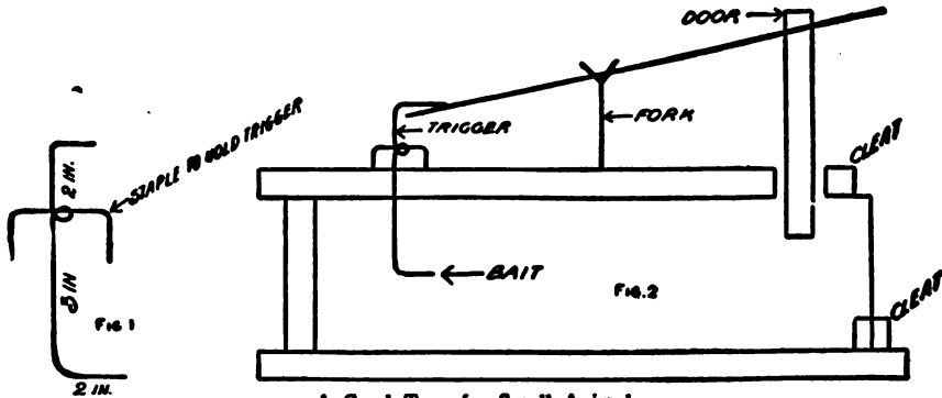
A Good Trap for Small Animals
