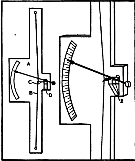
The Hygrometer
