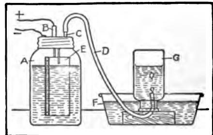
Hydrogen Generator
