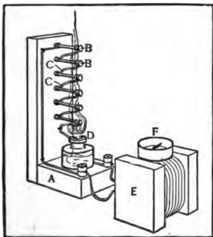
Thermo Battery
