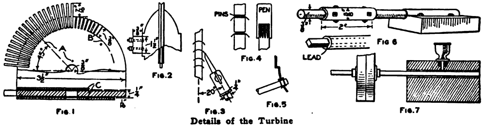
Details of the Turbine
