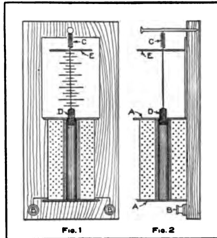
Battery Voltmeter Construction
