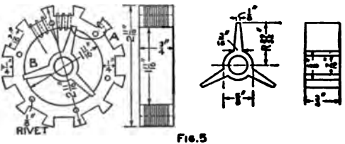
Armature-Ring Core, Its Hub and the Construction of the Commutator and Its Insulation
