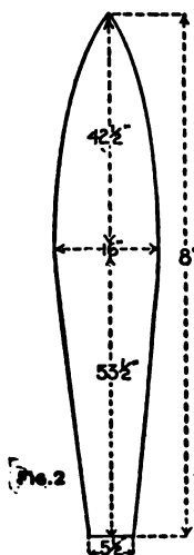
Fig. 2 Pattern and Parts to Make Balloon
