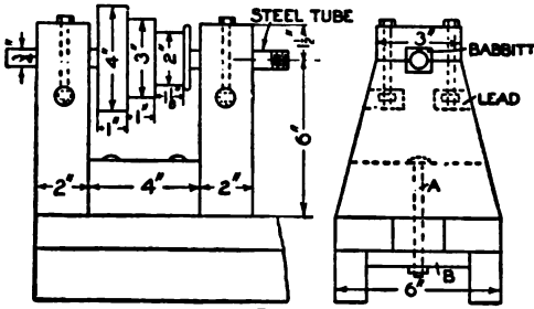
Fig. 6 Headstock Details
