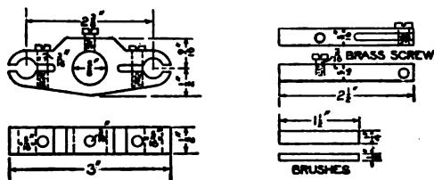
Fig. 8 The Insulated Brush Holder and Its Studs for Holding the Brushes on the Commutator
