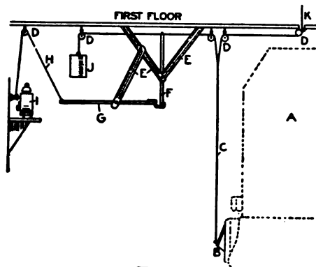
Draft Regulator
