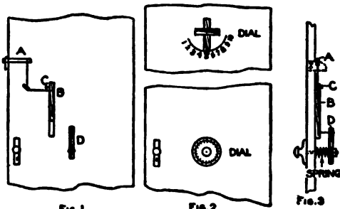
The Lock Parts
