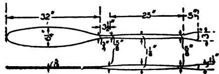
FIG. 13 A Single Paddle
