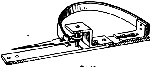
FIG. 13 Assembled Thermostat
