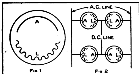
Electrolytic Rectifier and Connections
