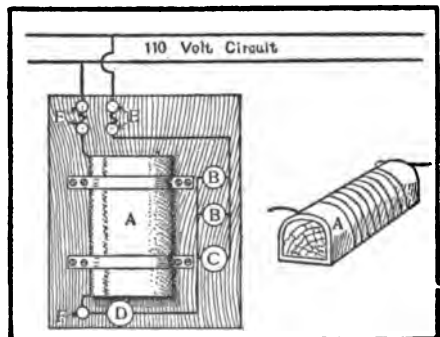
Electric Furnace
