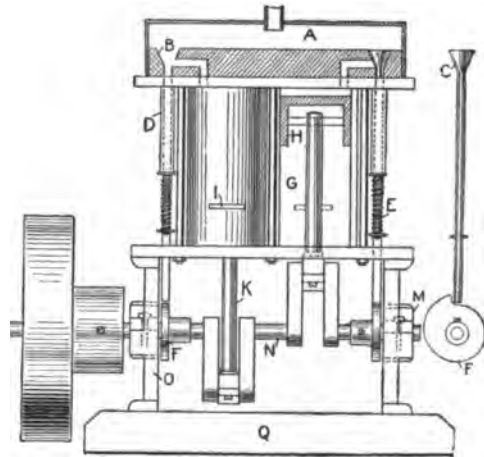
Engine Details
