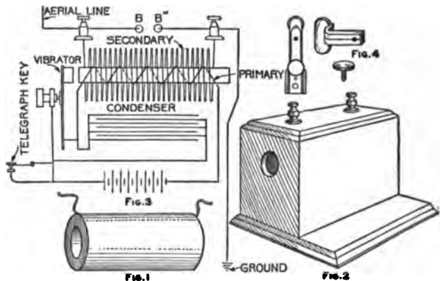
Jump-Spark Coil
