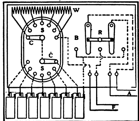
Motor Reverse and Controller
