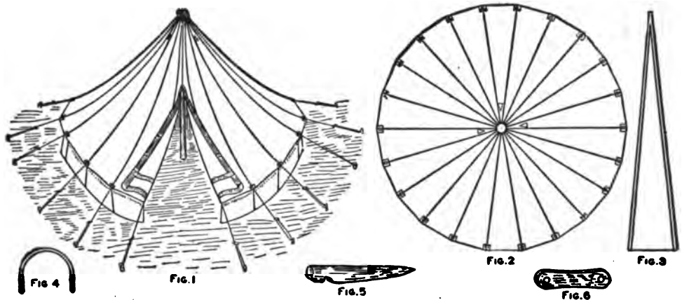
An Inexpensive Home-Made Tent
