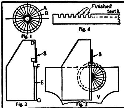
Making Model Wheels
