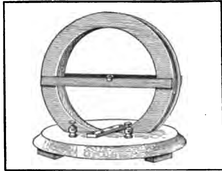
Tangent Galvanometer
